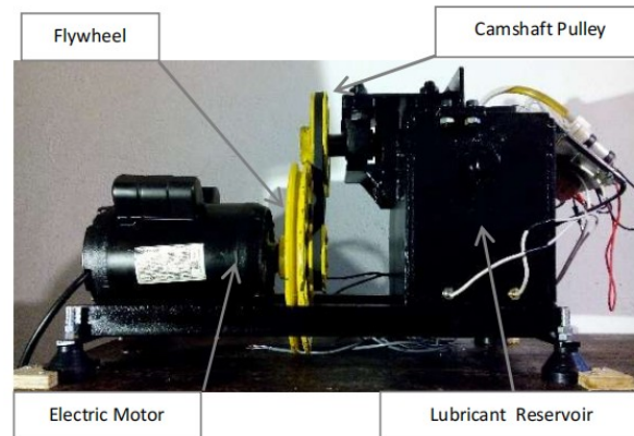
Figure 1: Direct Acting Mechanical Bucket Tappet Apparatus for Tribological Experiments.
